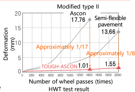
Modified type II Ascon TOUGH-ASCON Semi-flexible pavement
